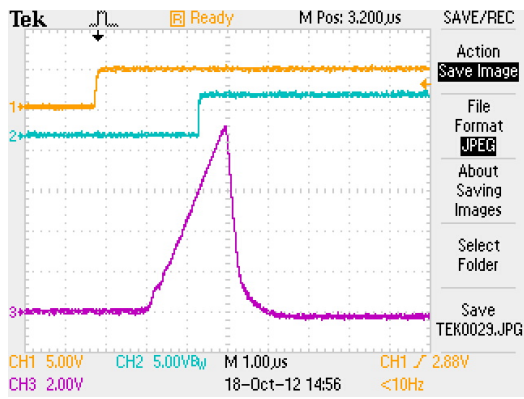
Figure 3. Simulated Arc. The fault occurs at 246 A. The switch opens in 690 ns; current peaks at 365 A.
