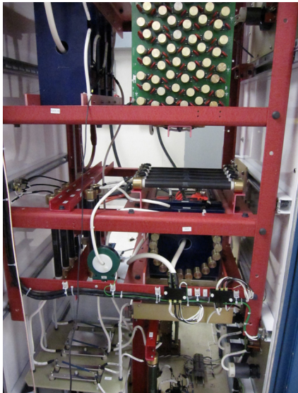
Figure 2. High Voltage Cabinet. Clockwise from top left: Switch Plate; Snubber Circuit; Grid and Screen Plates; Filter Capacitor; Storage Capacitor.
