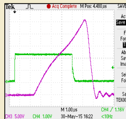
Fault Response of DTI Solid-State Circuit Breaker. Purple: Current, 200 A/div. Green: Command. The switch opens at 900 A, tripping in ~1.2 microseconds. Fault current is limited to ~1200 A.
