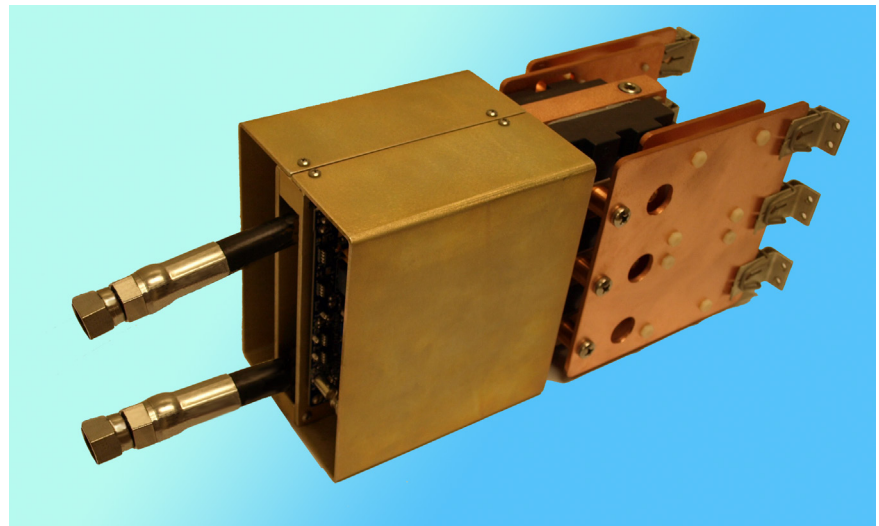
4.5 kV, 600 A Solid-State DC Circuit Breaker. This breaker is based on technology developed to protect radar and particle accelerators. This DC solid-state circuit breaker is comprised of two 4.5 kV IGBTs in series (for voltage margin). and has dimensions of 16”w x 8”d x 6”h.
