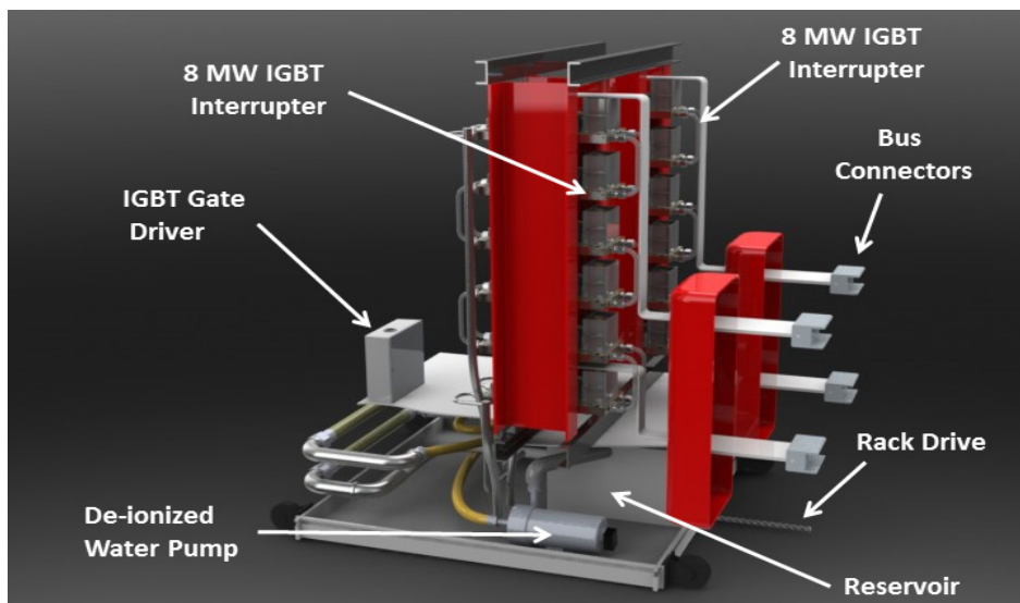
8 MW Solid-State DC Circuit Breaker. Conceptual drawing of a solid-state circuit breaker comprised of two 10 kV, 8 MW interrupters. Dimensions of 32" w x 32" d x 42" h.
