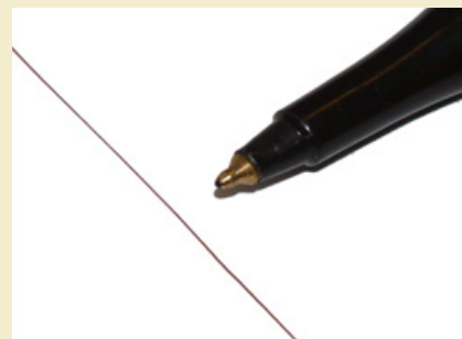
Fault Testing. #40 AWG arc test wire shown next to a ball point pen for scale. Shorting a 100 kV capacitor bank to ground through a 500 μH inductor and a length of #40 AWG wire leaves the wire intact, due to DTI's rapid fault detection and current interruption circuitry.
