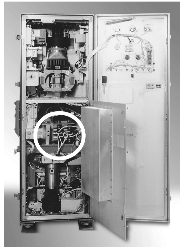
Figure 3: AN/SPG-60 transmitter with DTI solid state modulator installed in middle cabinet.
