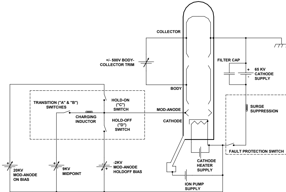
Figure 8: Schematic of NRL gyrokystron modulator.
