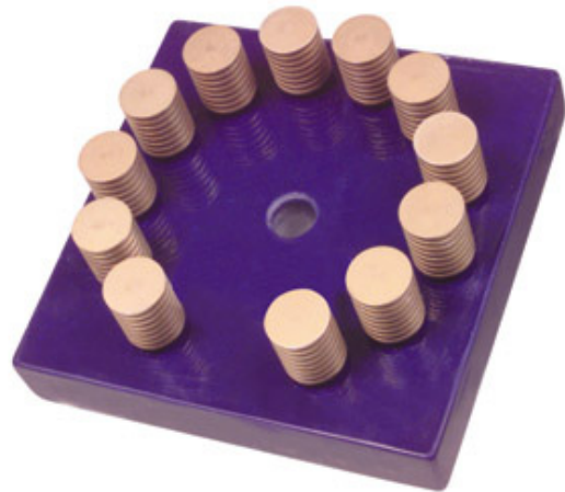
Figure 1: 9kV, 30A Solid State Switch Module Approximately 7" x 7" x 3"
