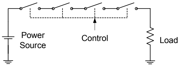
Figure 2: Solid state modulator components. The switches are in series.
