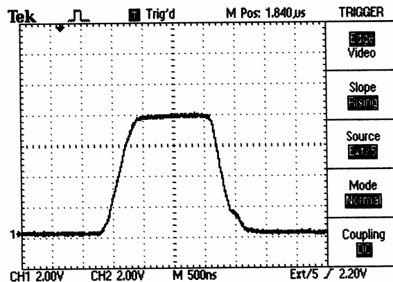
Figure 5: Transmitter pulse 8kV, 100kHz, 1.5 \mu s
