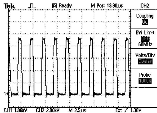
Figure 7: 4.5kV, 400kHz pulse
