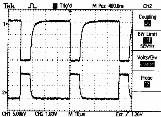
Figure 4: AN/SPG-60 train, 15kV, 25 kHz, 8 \mu s
