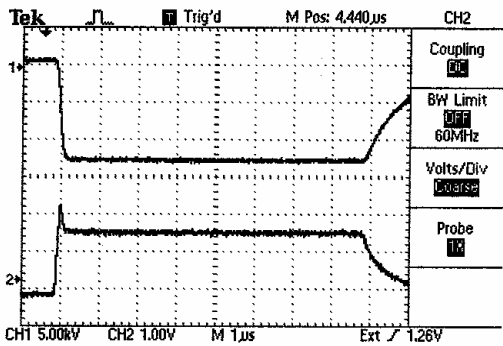
Figure 6: AN/SPG-60 Pulse, 13.5kV, 25 kHz, 8 \mu s
